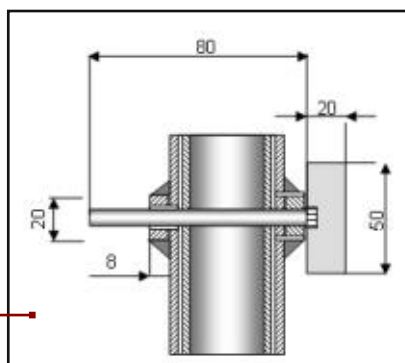
Constructional detail A
