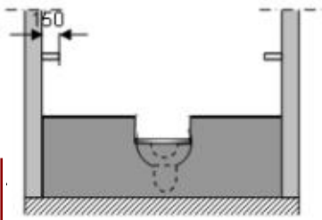
Constructional Detail
